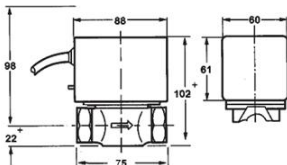
V4043BSPP/BSPT
