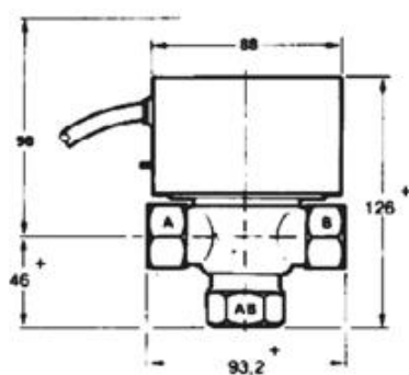
V4044 BSPP/BSPT
